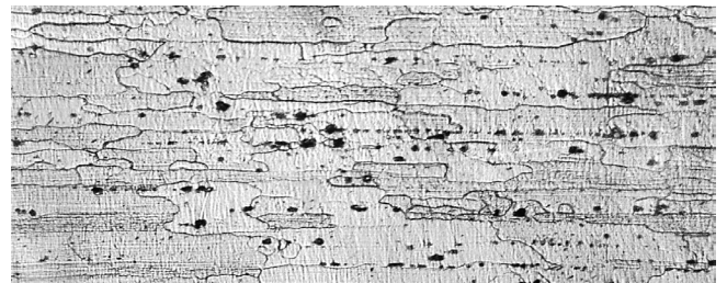
Figure 3-11. Cross-Section of 7075-T6 Aluminum Alloy
